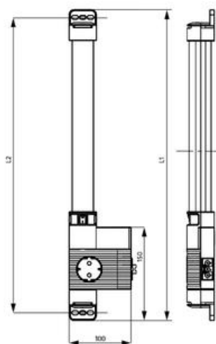
LED 121 (Size 1) L1 = 500 mm L2 = 475 mm
